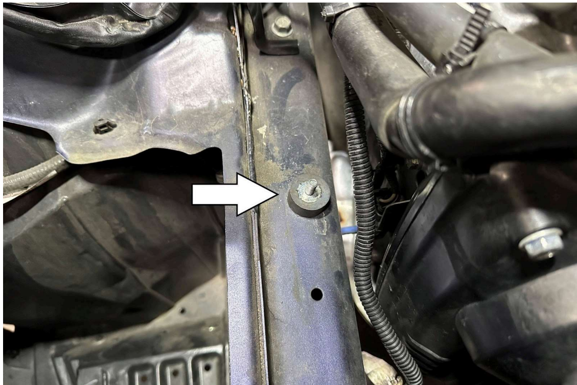
10. Install the 1/2" vibration mount onto the frame rail.
