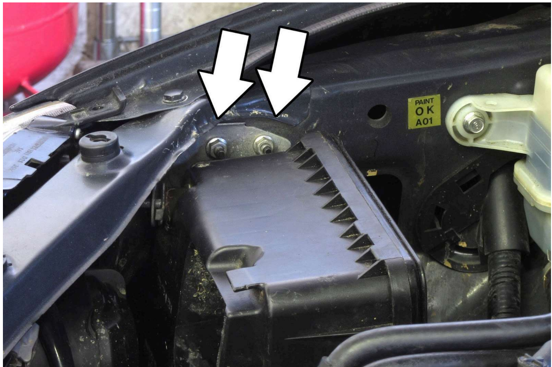
8. Remove the two nuts securing the lower air box assembly.
