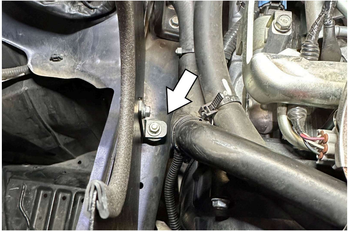
15. Position the heat shield onto the ½" vibration mount installed in step 10 and secure it using the provided nut and washer.
