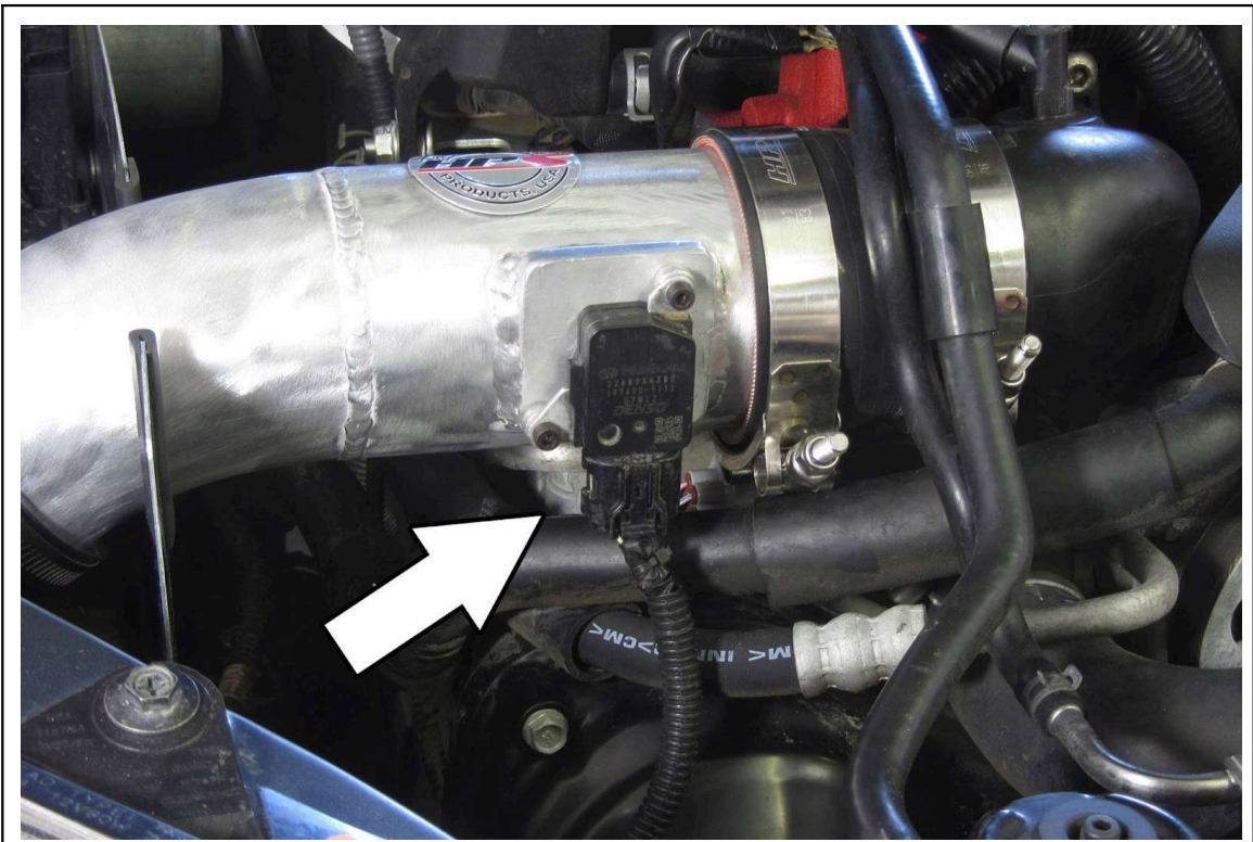
19. Reconnect the MAF sensor.
