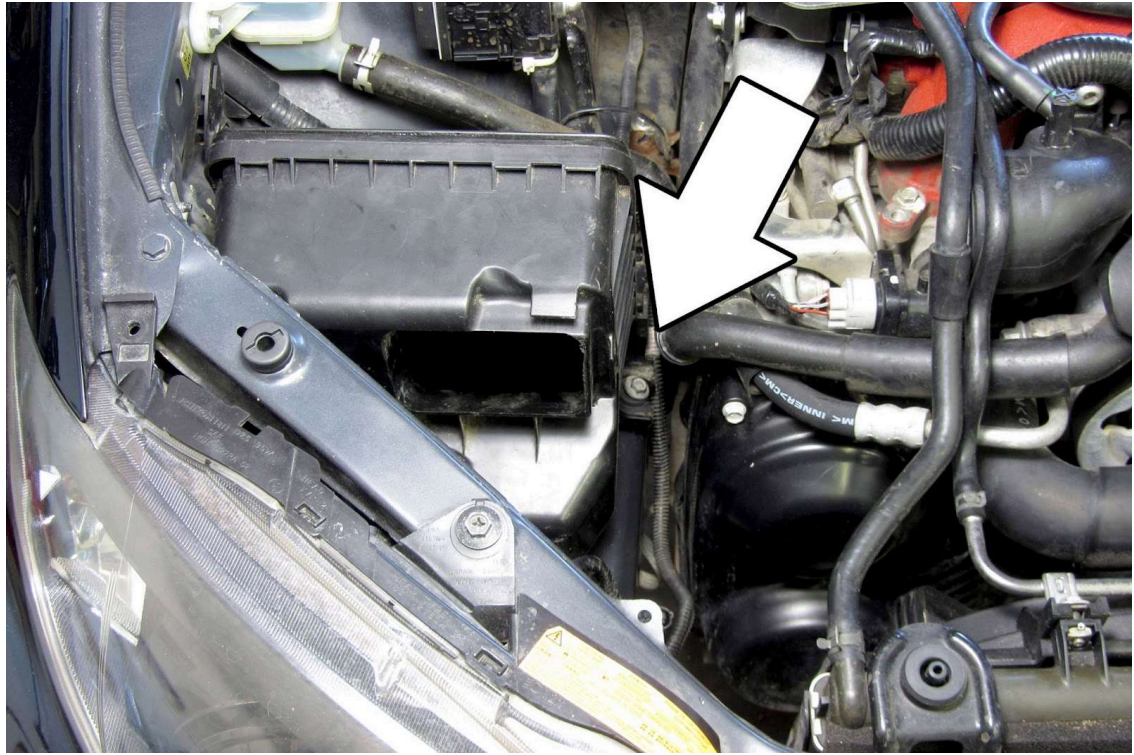
7. Remove the bolt securing the lower air box assembly to the frame rail.
