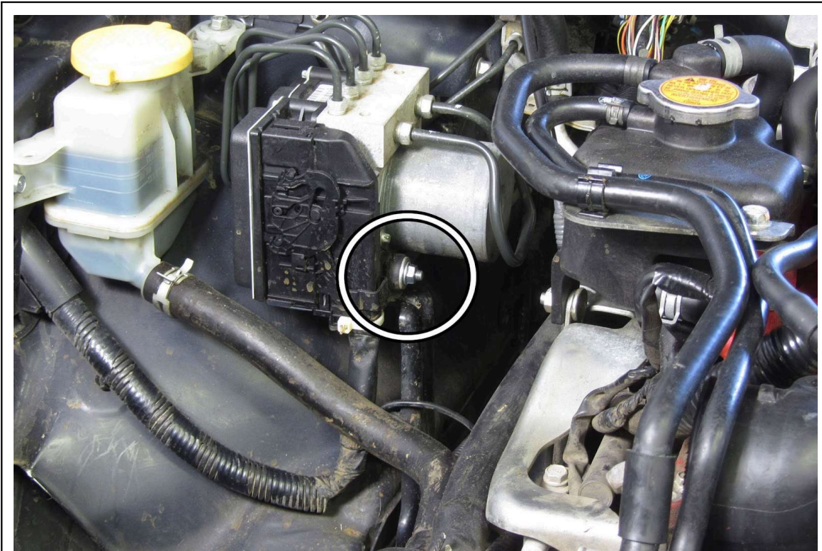
11. Use a 10mm wrench to remove the nut on the ABS unit.
