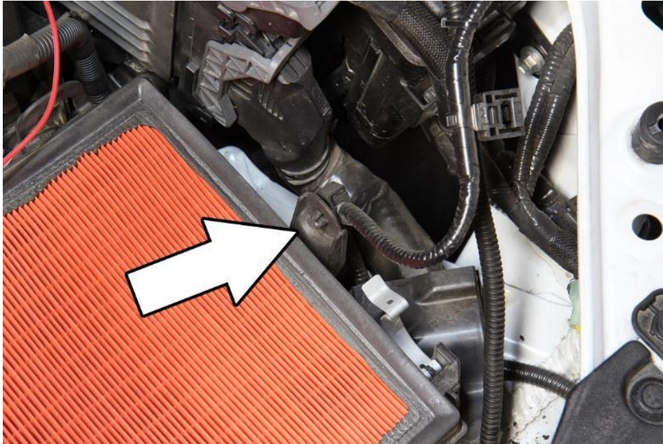
8. Disconnect the harness clip from the lower air box assembly.
