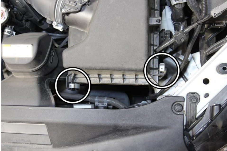
5. Disconnect the two retaining clips securing the upper air box assembly.
