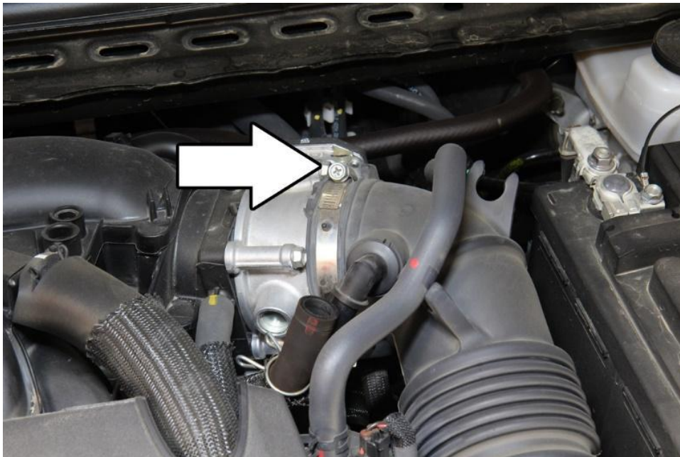
6. Loosen the hose clamp securing the intake tube from the throttle body.
