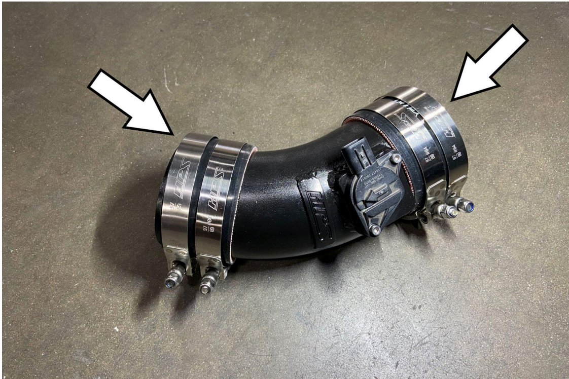
19. Loosely place the provided couplers and clamps onto both ends of the intake pipe. Tip: Slide the coupler shown on the left side of the image completely onto the intake pipe.
