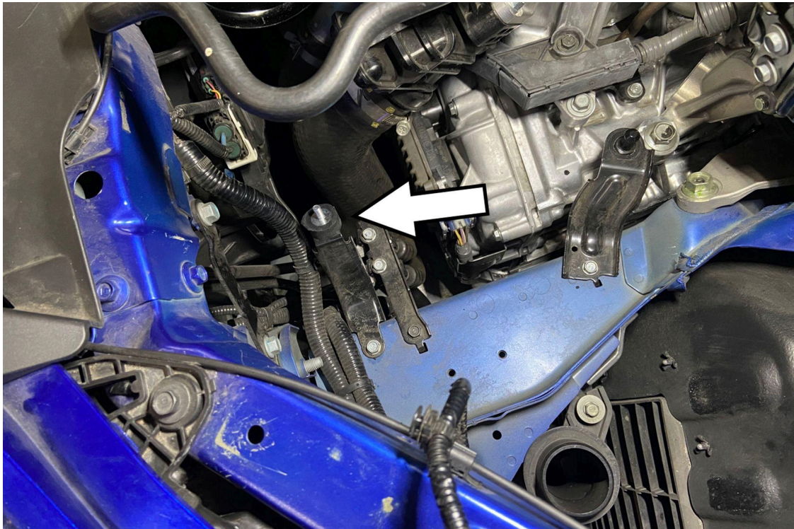
7. Install the provided 1/2" rubber vibration mount onto the front factory lower air box mount.
