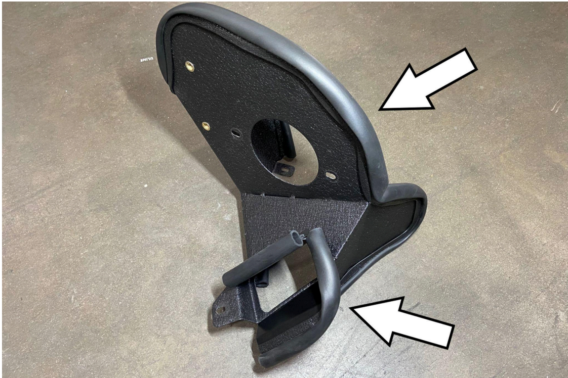
11. Install the provided bubble edge trim onto the HPS upper heat shield in the areas shown.
