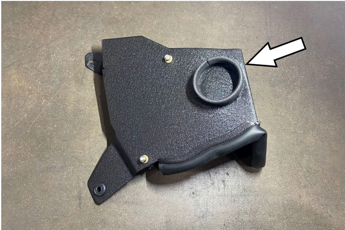
9. Install the thin edge trim onto the circular section under the lower heat shield.
