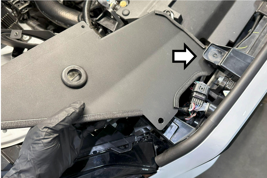
13. Place the air inlet heat shield into position. Be sure that the section indicated is positioned below the stock air duct mounting point.
