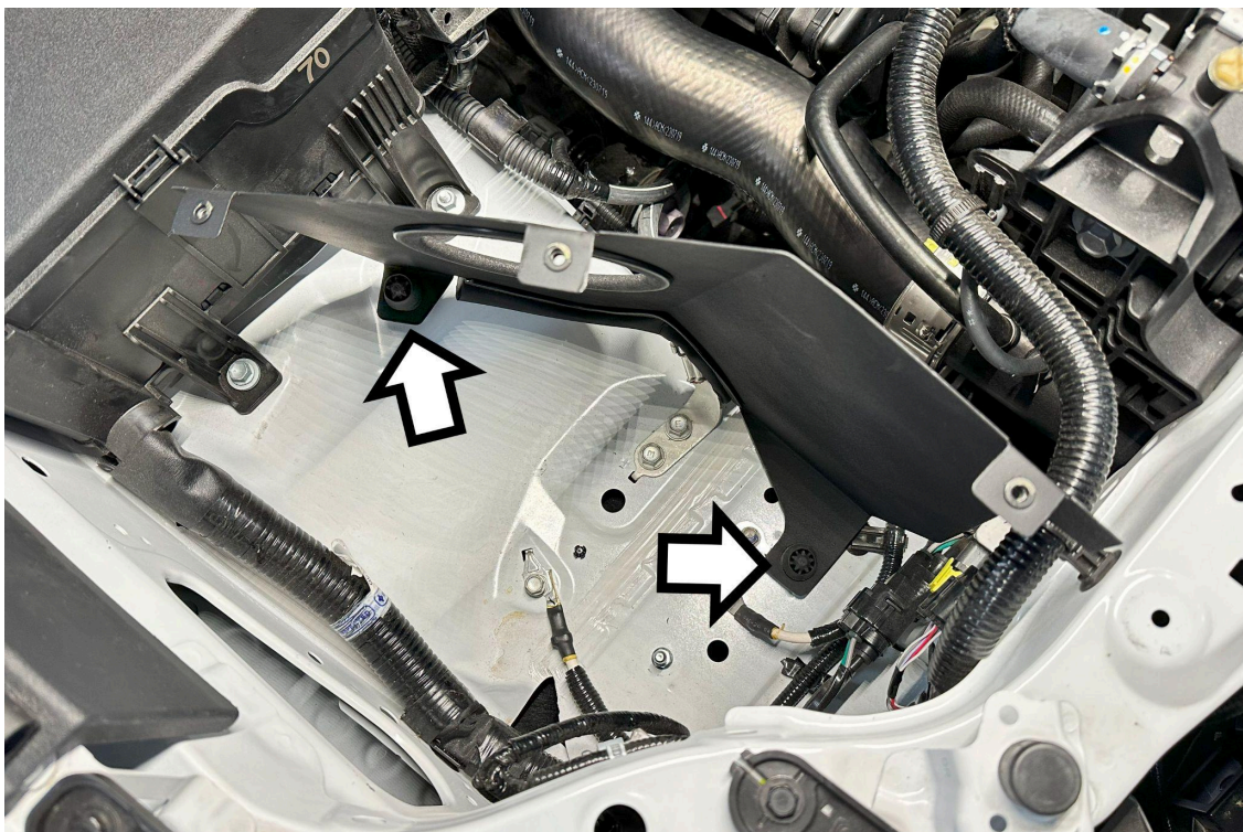
10. Carefully place the main heat shield into the engine bay and push the rubber grommets onto the factory mounting points.
